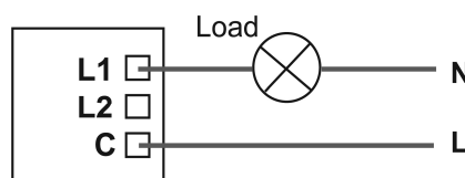
Figure 1. Using a 1 or 2-way dimmer switch
