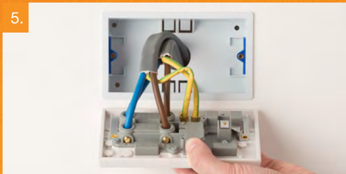
5. There will generally be three different wiring configurations. This photo shows a single wire of each colour connected to each terminal.
