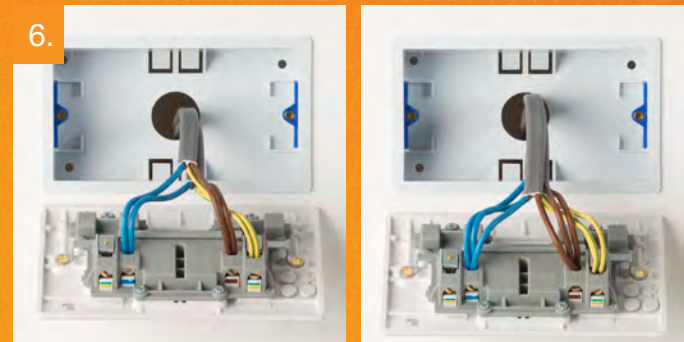
6. Alternatively, there could be two or three wires of each colour connected to each terminal.
