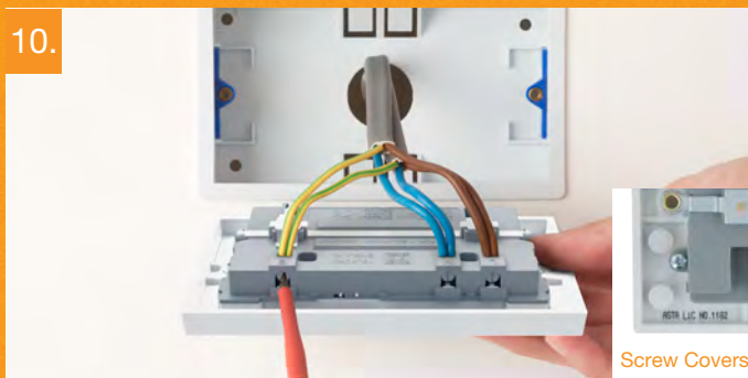
10. Make sure that the wires are fully inserted into the terminal and that no bare copper wire is visible. Tighten the screws securely onto the copper wire, not the outer sheathing. Before fixing remove screw covers from rear.
