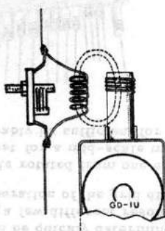
Inductive coupling to a coil
